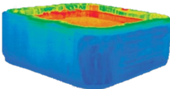
Infrared Heat Map – Bullfrog Spa
